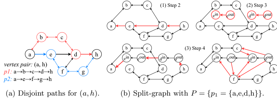
Fig. 1: Examples of disjoint paths and split-graph.
