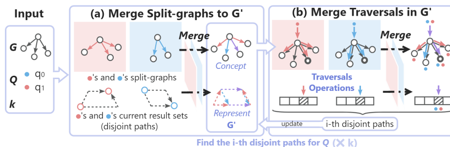
Fig. 2: Framework of ShareDP. Colored balls (e.g., the blue ball for query q_0 ) represent queries. Each iteration identifies a path for each query by conducting a combined search on a merged split-graph G' . See Sec. 5.1 for details.
