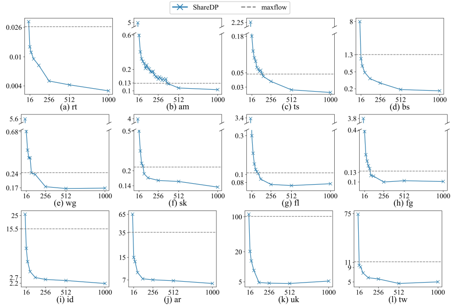
Fig. 4: Running time when varying the number of k DPs with k=10 .
