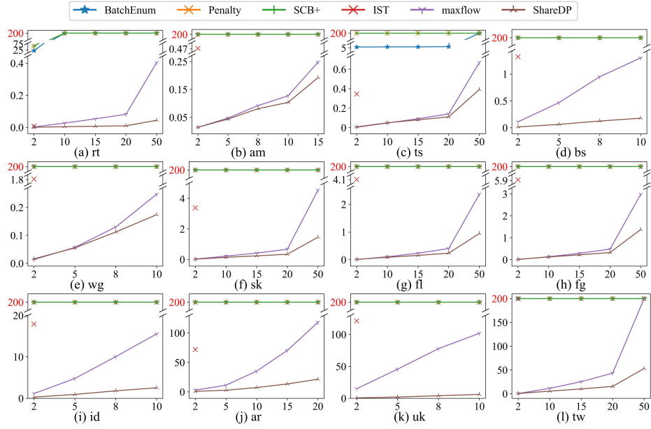
Fig. 3: Running time when varying k .
